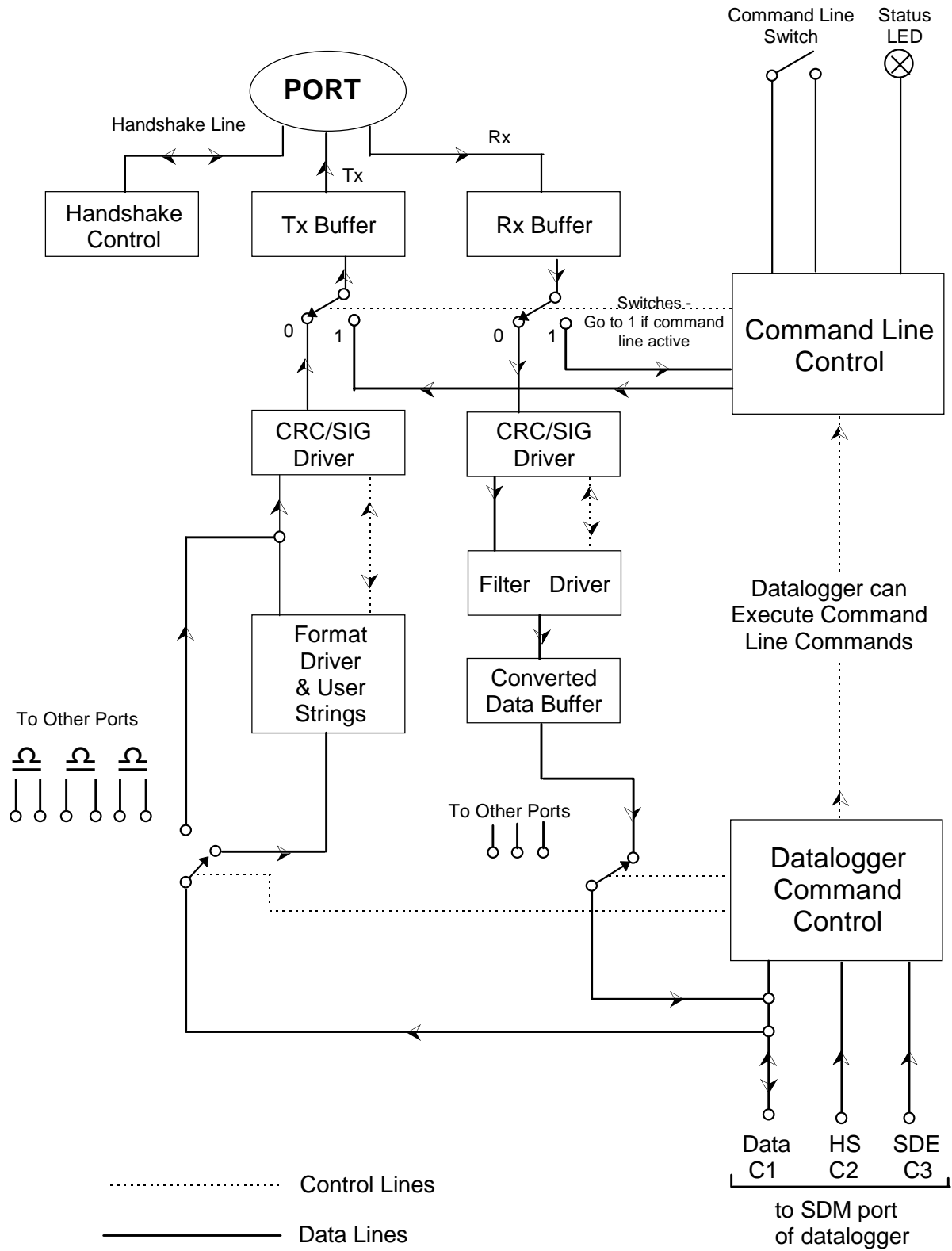
FIGURE 1. Schematic Diagram of the SDM-SIO4
