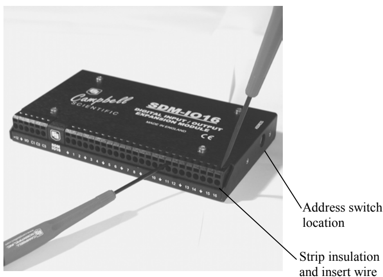
FIGURE 4. Use of Terminal Blocks
