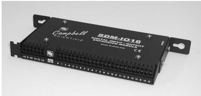
FIGURE 1. SDM-IO16 (with mounting brackets)
