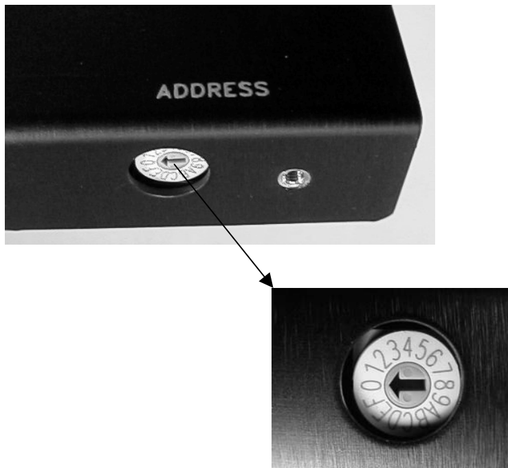
FIGURE 5. Address Selection Switch
