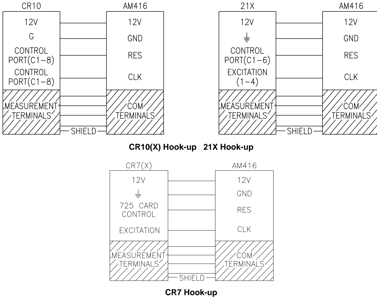
FIGURE 2. Hook-up Diagrams for Datalogger - AM416 Connections
