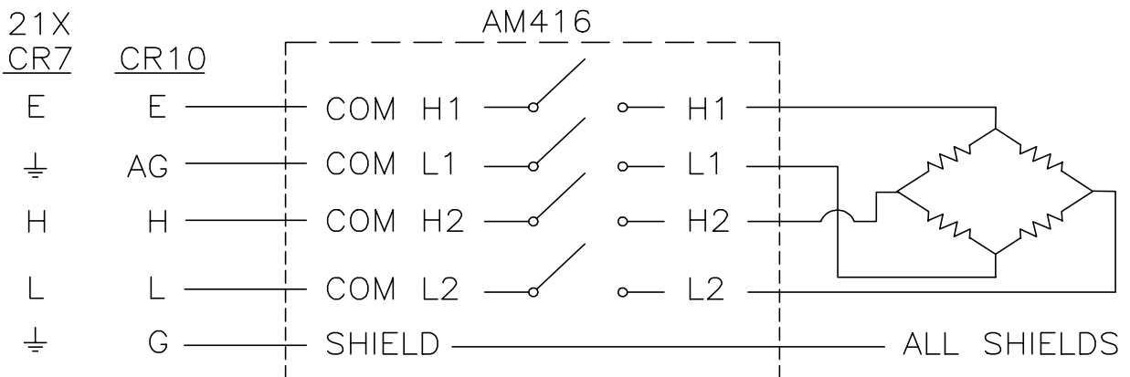
FIGURE 13. Differential Measurement with Sensor Excitation
