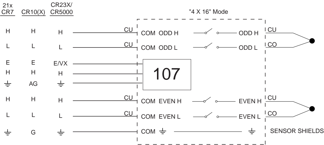
FIGURE 18. Differential Thermocouple Measurement with Reference Junction at the AM16/32.
