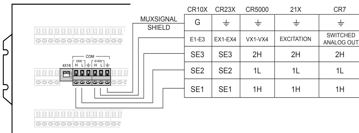
FIGURE 5. Typical AM16/32 to Datalogger Signal Hookup (4x16 Mode)
