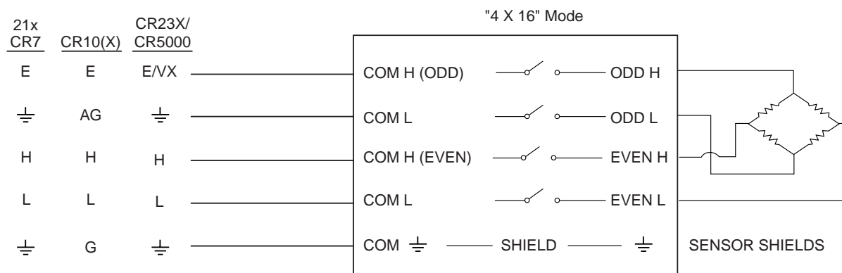
FIGURE 15. Full Bridge Measurement
