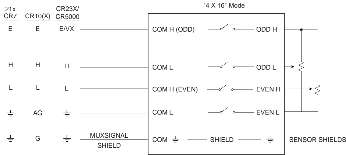
FIGURE 13. Potentiometer Hook-up and Measurement
