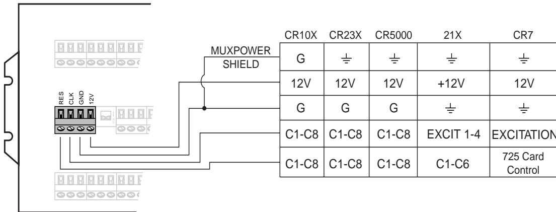
FIGURE 3. AM16/32 to Datalogger Power/Control Hookup
