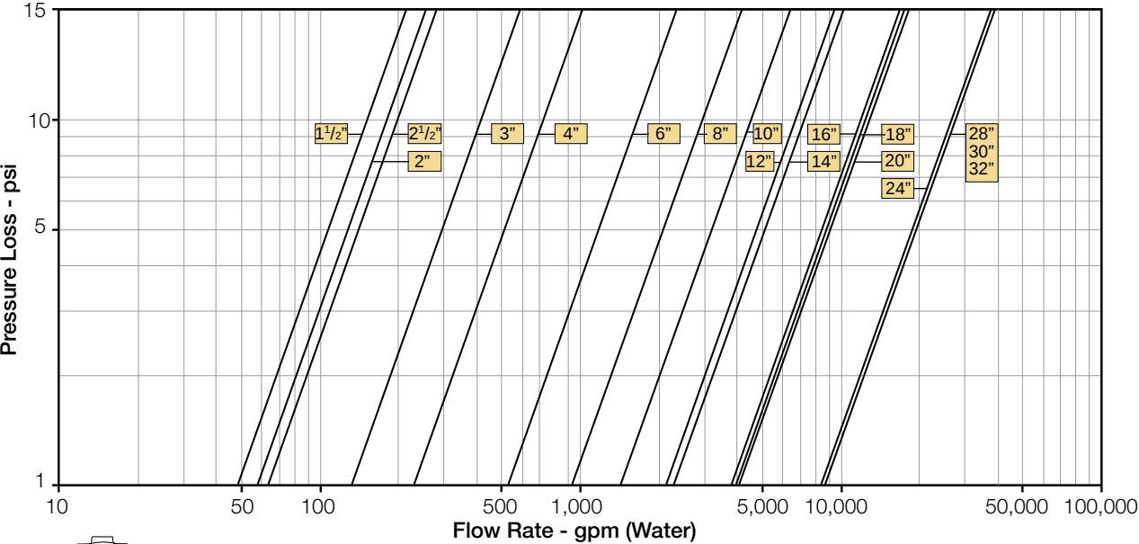
Angle Pattern, Flat Disc
