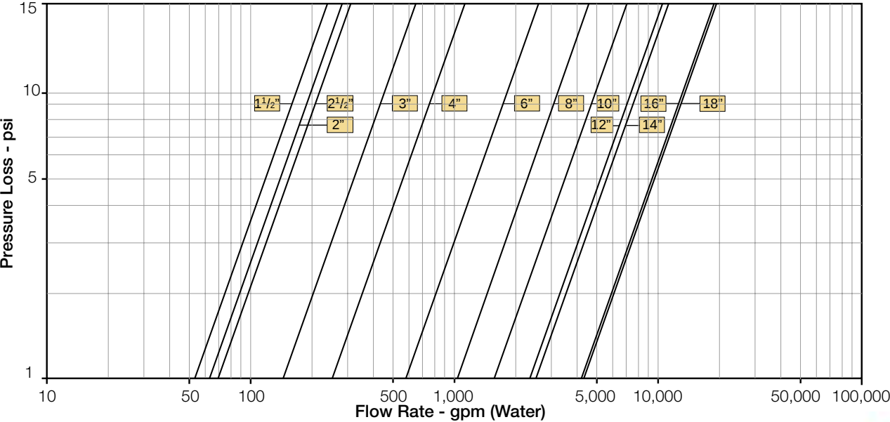
Angle Pattern, Flat Disc
