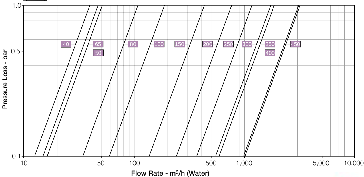
Angle Pattern, Throttling Plug (U-Type)
