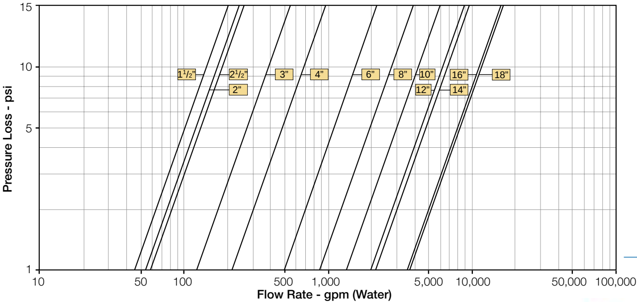
Angle Pattern, Throttling Plug (U-Type)
