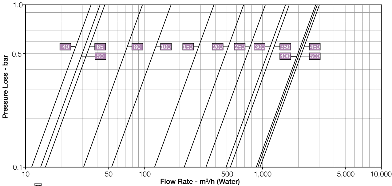
Y Pattern, Throttling Plug (U-Type)
