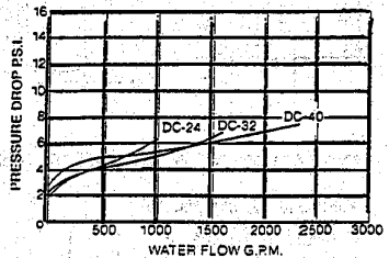
Lawler Double Check Backflow Preventer
