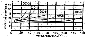
Lawler Double Check Backflow Preventer
