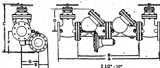
INSTALLATION DIMENSIONS (inches)
