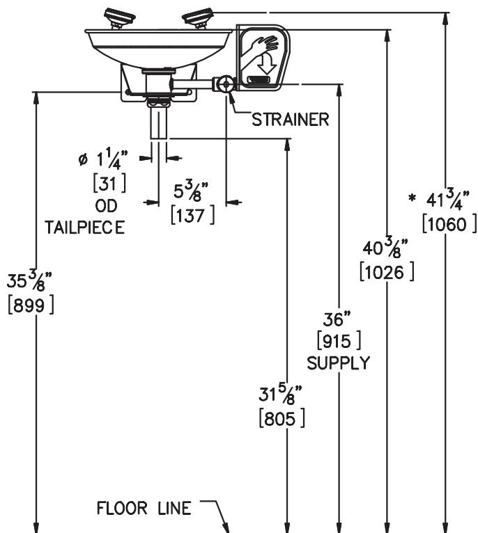
MOUNTING DETAIL
