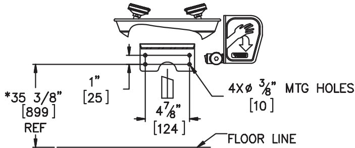
MOUNTING DETAIL
