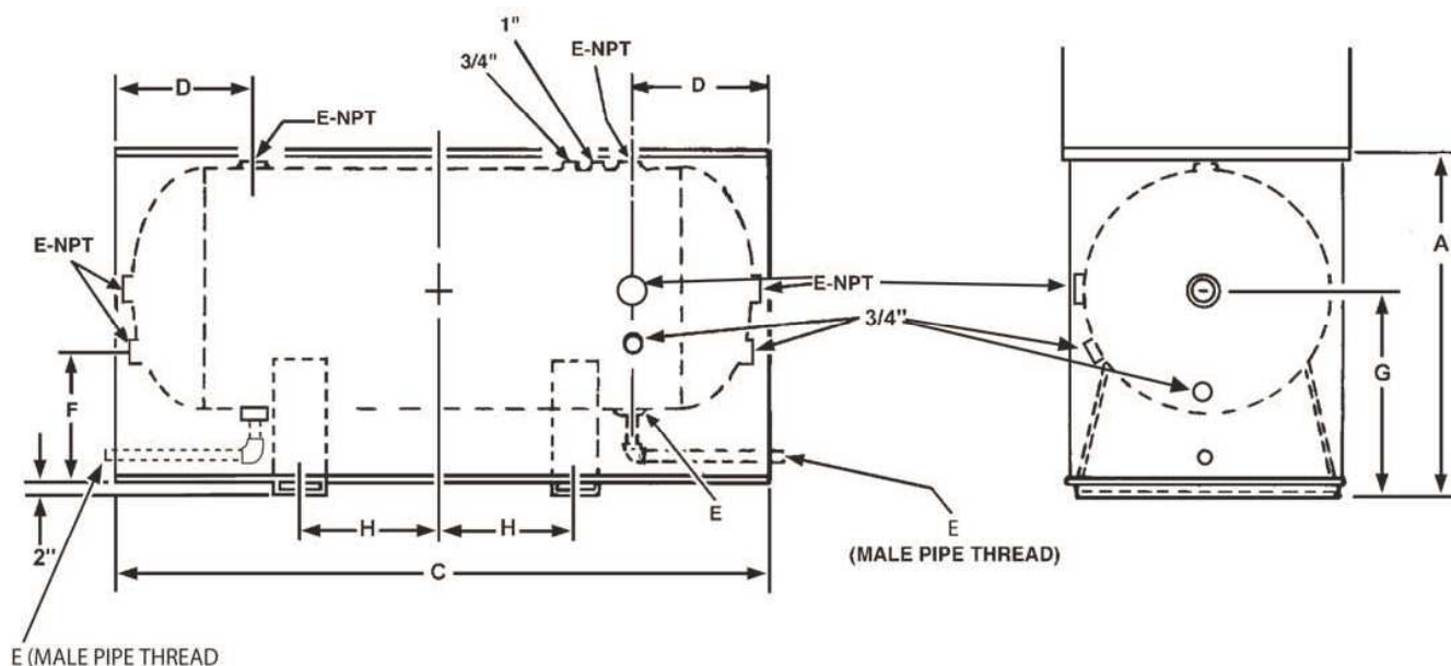
TJH-200 THRU TJH-1000 FIGURE 2.
