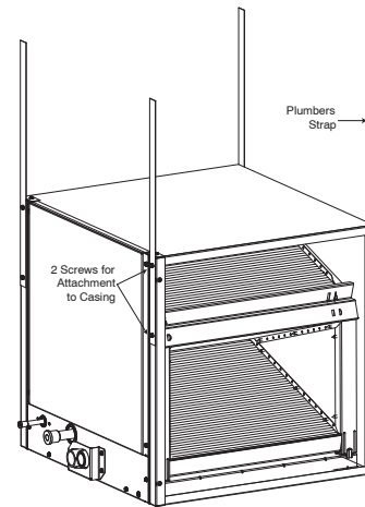
Fig. 7 - CNPHP Suspension with Plumbers Strap
