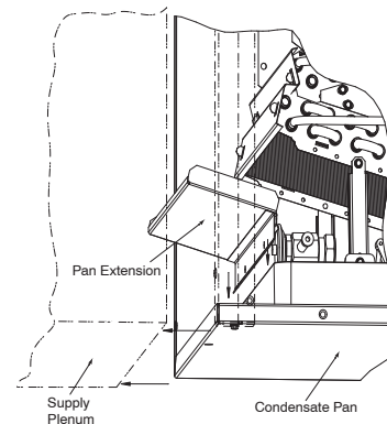
Fig. 2 - Horizontal-Left Installation of Pan Extension
