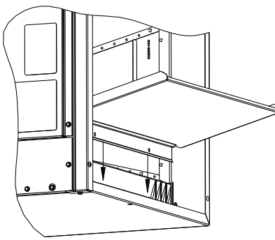
Fig. 3 - Horizontal-Right Installation of Pan Extension
