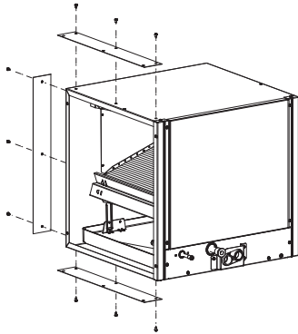
Fig. 5 - Mount Attachment Plates
