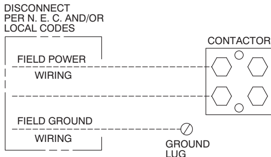
Fig. 6 - Line Connections
